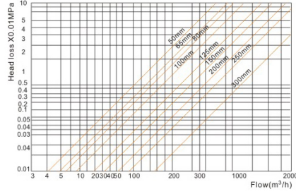
Head Loss Curve
